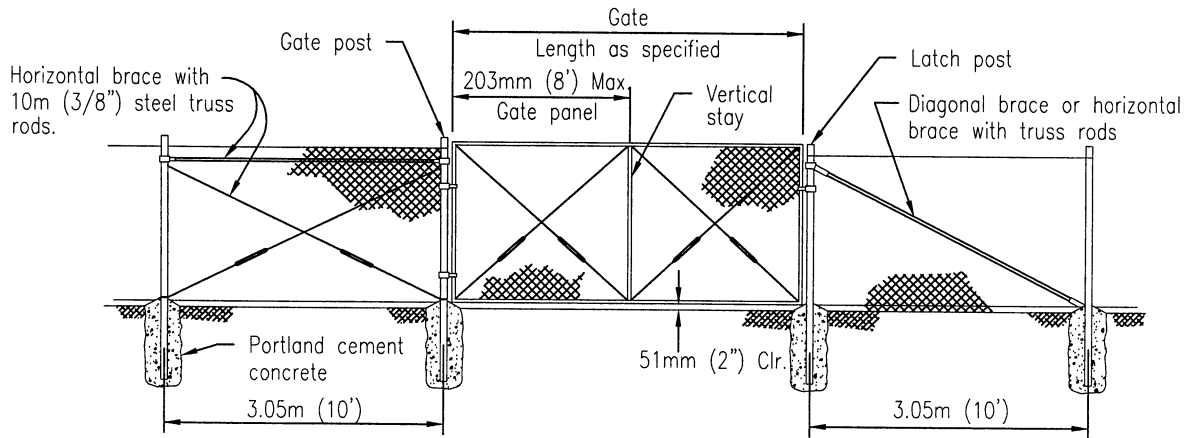
GATE ASSEMBLY
