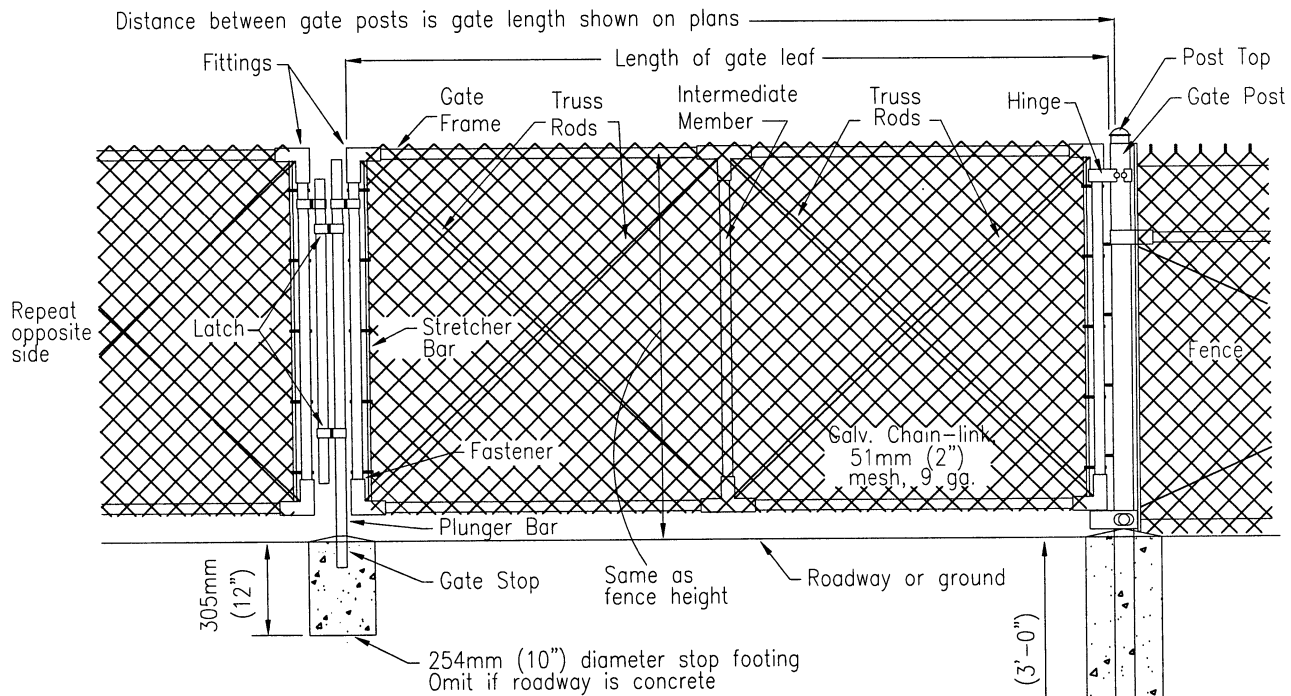
HALF ELEVATION DOUBLE SWING GATE
